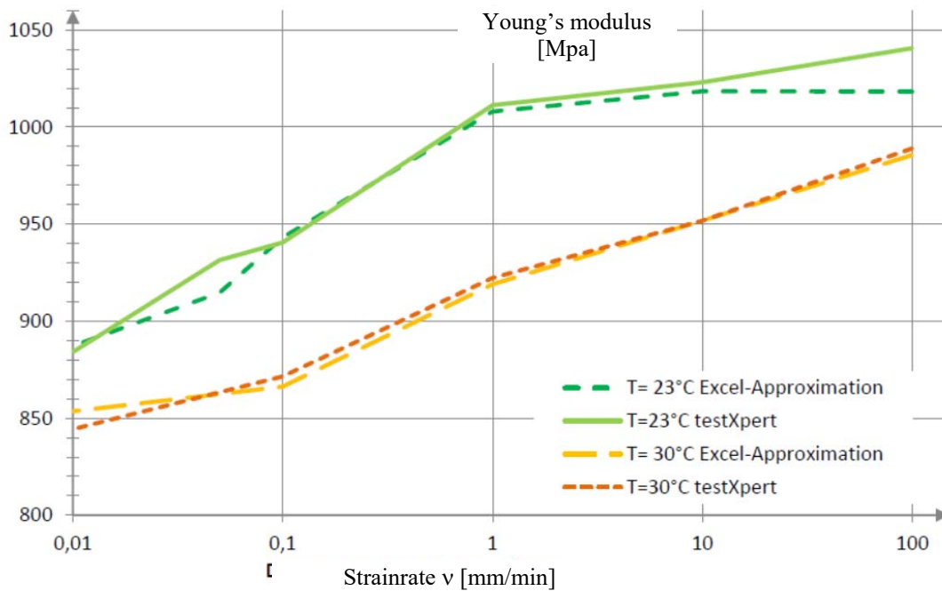
Figure 14: Young's modulus (uniaxial) for two temperature levels, plotted against the measured strain rate levels between 0.01 and 100 mm/min, determined by the testing software testXpert as well as calculated from single values with the software EXCEL [2].
