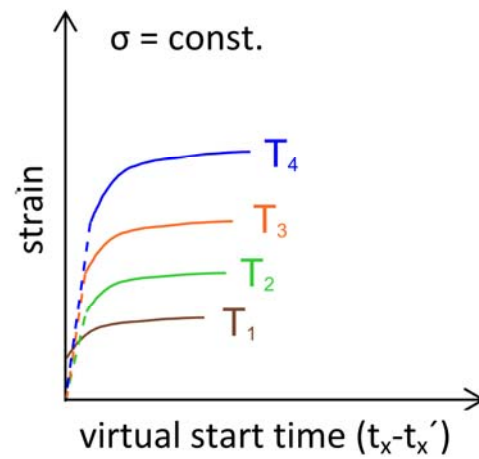
Figure 19: SIM – schematic procedure - step 3: horizontal shift of the initial (start) time
