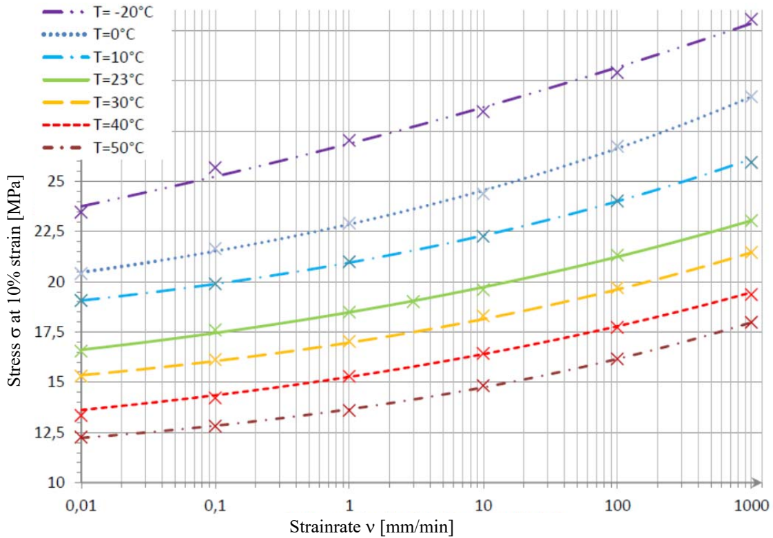
Figure 15: Stress at 10% strain by means of approximation function for the investigated temperature levels logarithmically plotted against the constant strain rate (crosshead speed) between 0.01 and 1000 mm/min [2].
