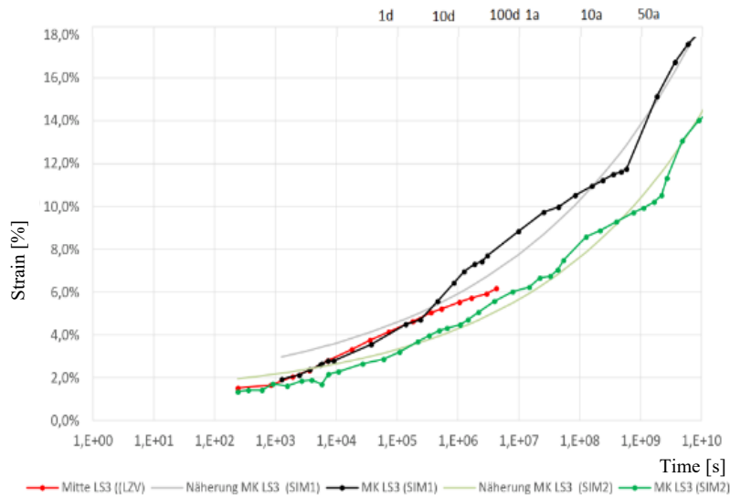
Figure 22: Evaluated curves of load level 3 [3]
