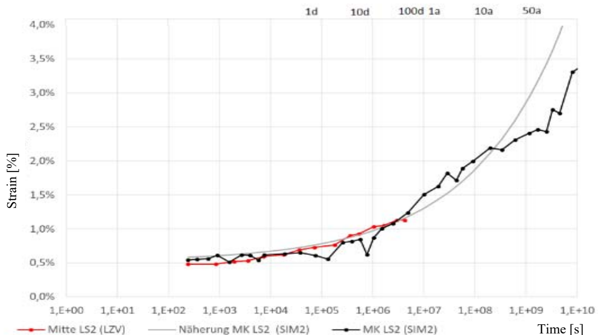
Figure 21 Evaluated curves of load level 2 [3]
