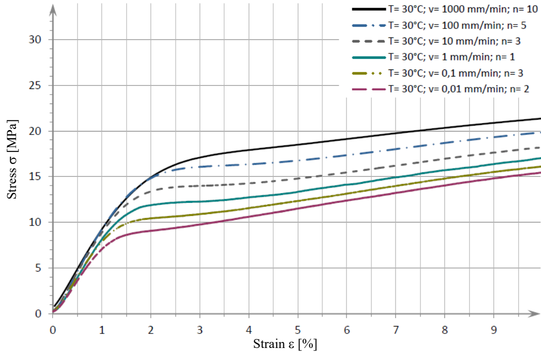
Figure 11: Stress-strain curves (mean values) for T = 30^{\circ}\text{C} [2]
