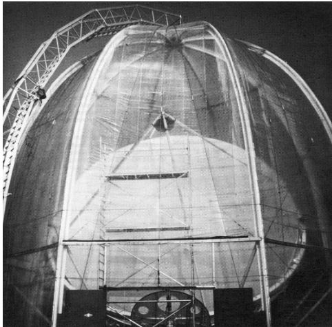
Figure 1: Dome - Temporary ETFE foil construction at the International Solar Forum 1980 in Hamburg [6].
