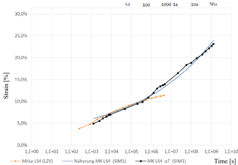
Figure 23: Evaluated curves of load level 4 [3]
