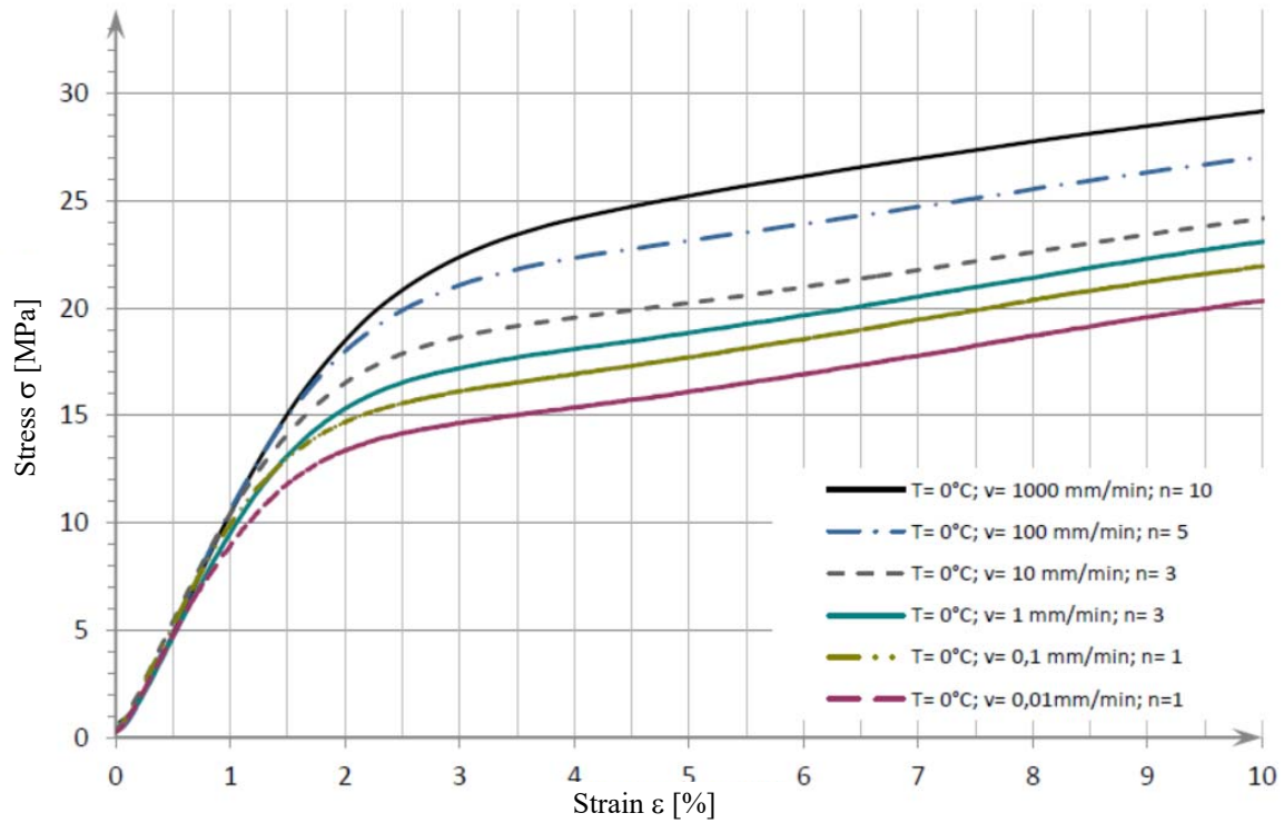
Figure 9: Stress-strain curves (mean values) for T = 0^\circ\text{C} [2]
