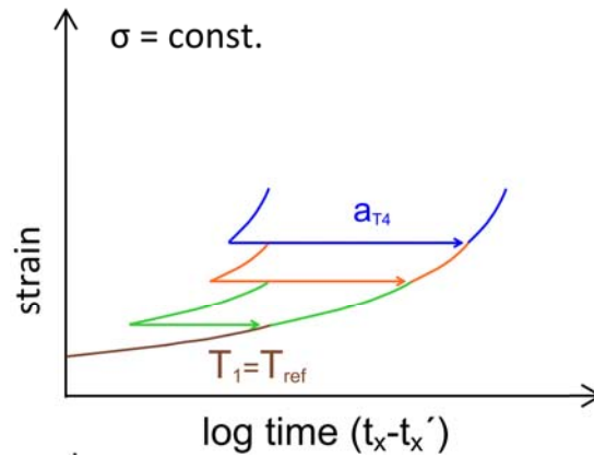
Figure 20: SIM – schematic procedure – step 4: logarithmic shift of the initial (start) time based on the Arrhenius-equation
