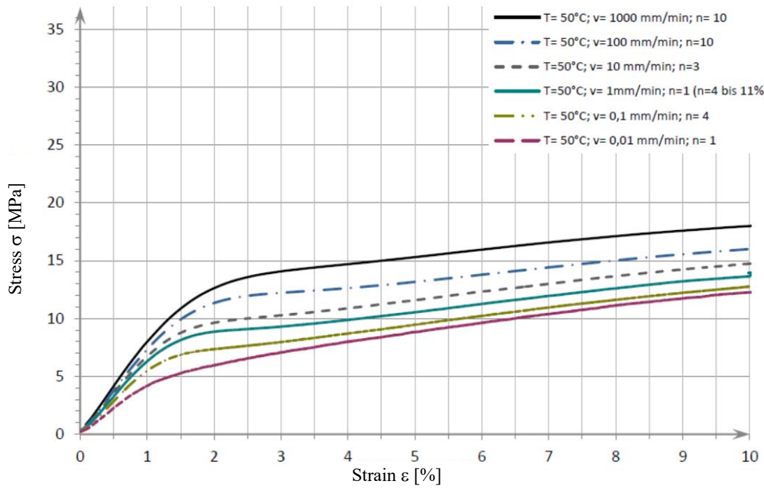
Figure 13: Stress-strain curves (mean values) for T = 50^{\circ}\text{C} [2]
