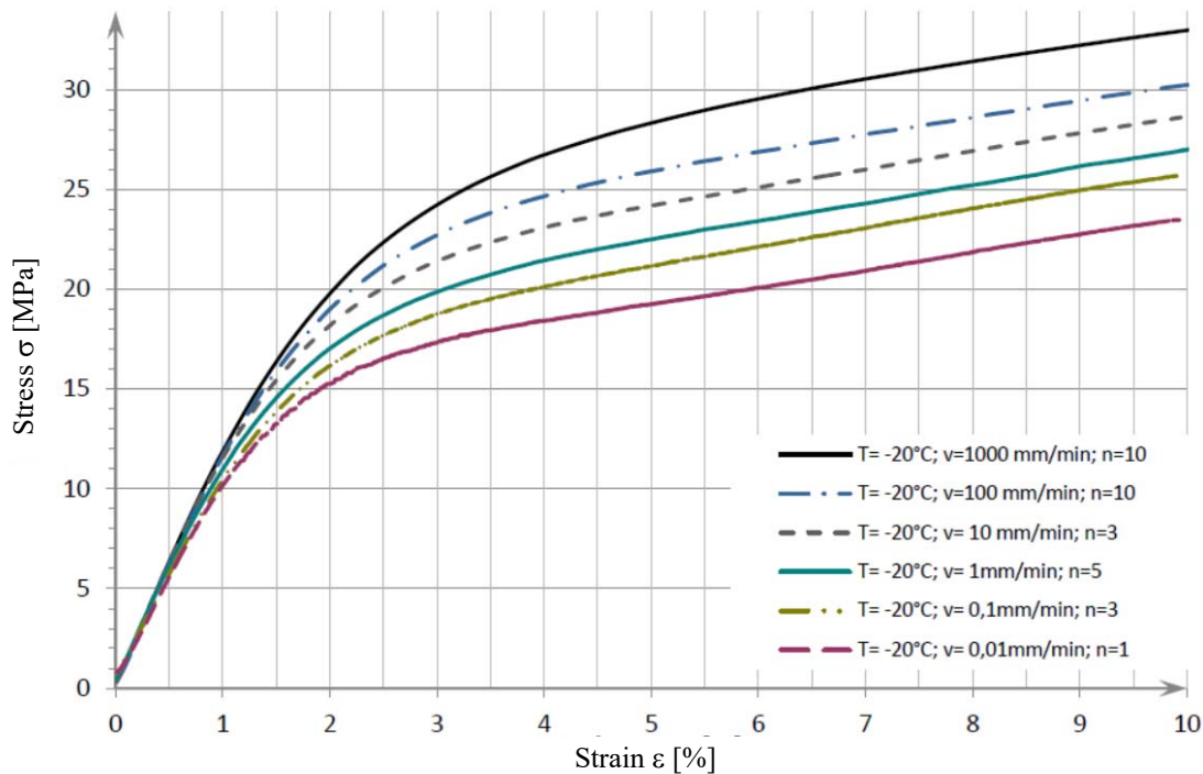
Figure 8: Stress-strain curves (mean values) for T = -20^{\circ}\text{C} [2]
