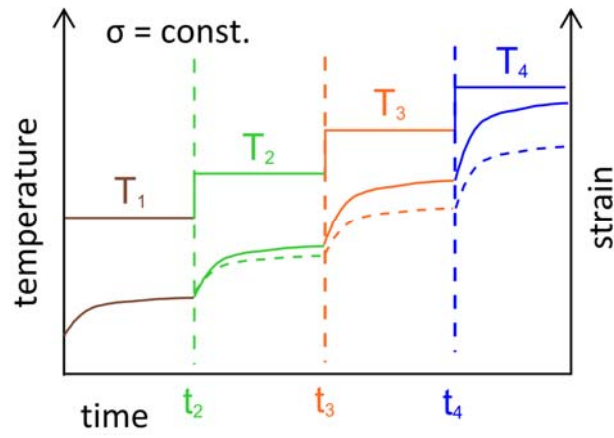
Figure 17: SIM – schematic procedure - step 1: stepped strain-time diagram
