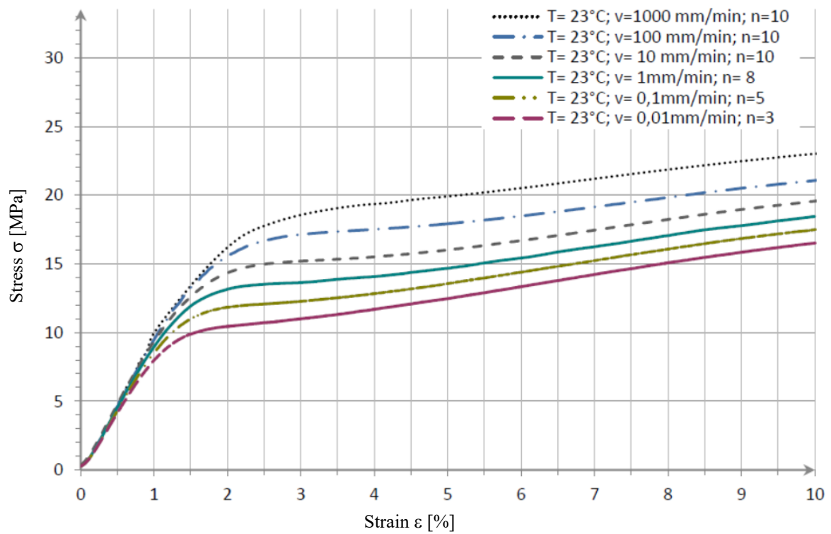
Figure 10: Stress-strain curves (mean values) for T = 23^\circ\text{C} [2]
