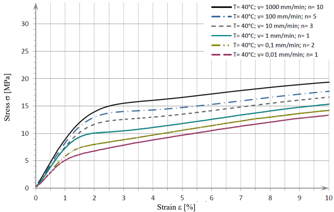
Figure 12: Stress-strain curves (mean values) for T = 40^{\circ}\text{C} [2]
