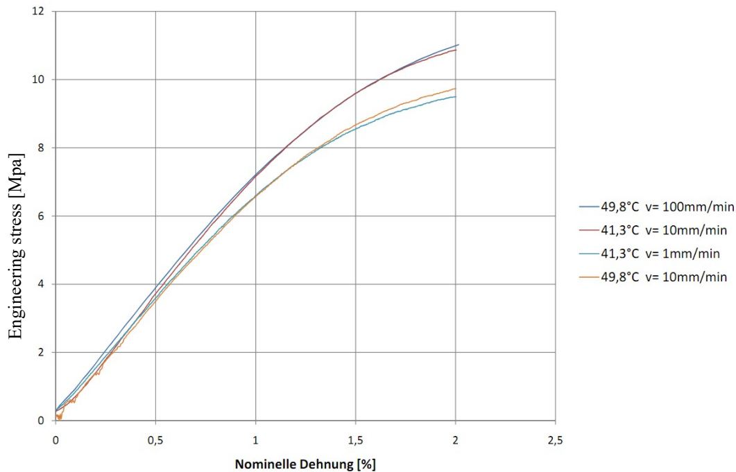
Figure 6: Relationship of changes in temperature and strain rate in case of ETFE-foils (NOWOFOLON ET6235Z) in the nominal strain range \varepsilon = 0\text{--}2\% [2]
