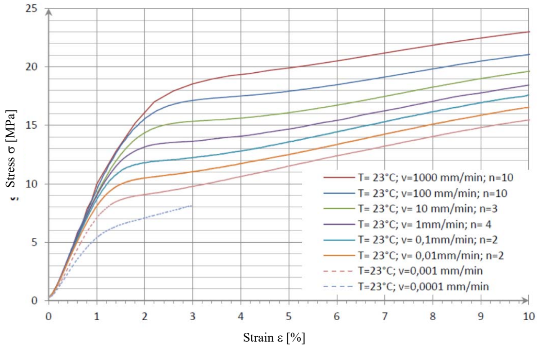
Figure 16: Extension to the stress-strain curves for strain rates v = 0.001 and 0.0001 mm/min (mean value curves) determined by means of Arrhenius -function and derived time-temperature shift factors [2].
