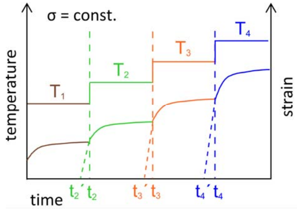
Figure 18: SIM – schematic procedure - step 2: Application of the Boltzmann's superposition principle
