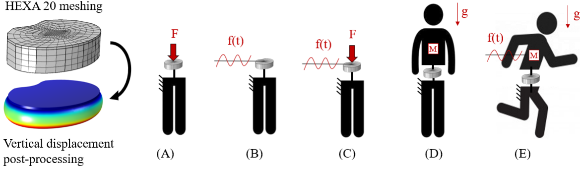
Figure 4: Geometry of IVD and post-processing mapping (left) and boundary conditions apply on the upper side of L4/5 IVD (right).
