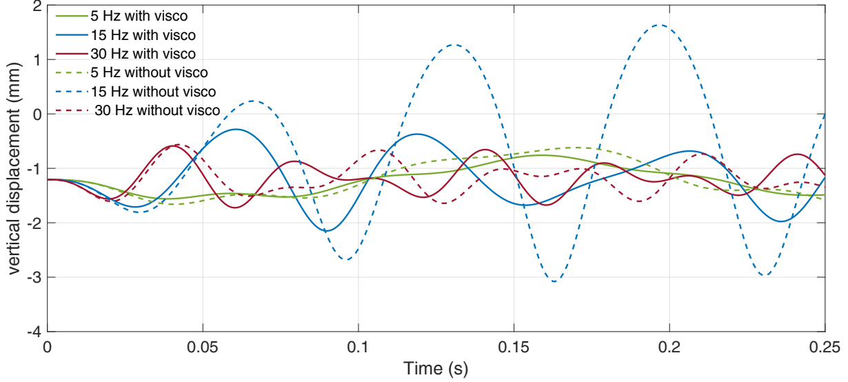
Figure 7: Dynamic analysis (E). Influence of the excitation frequency and of the viscoelastic contribution.
